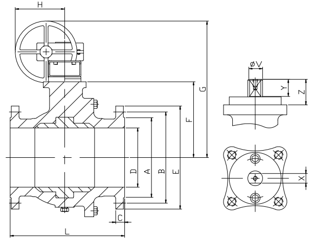
FIG.ZG 16 TTTGV CL150 6"-12"
