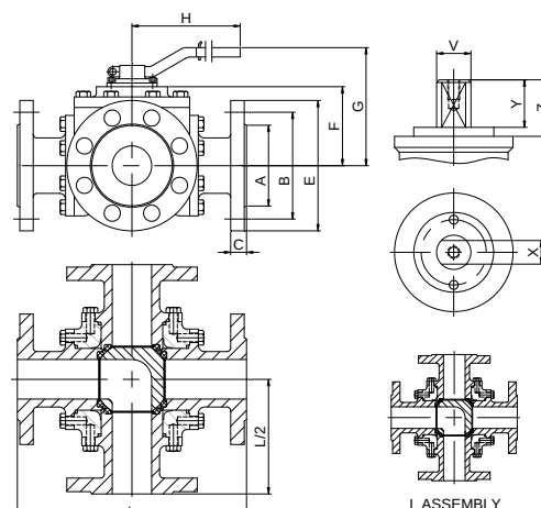
FIG.Z 74 TTT CL150 1"-8" L
