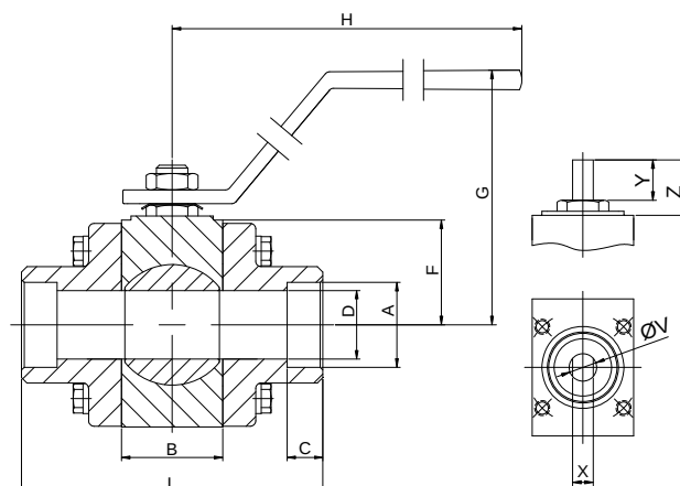
FIG.K 809 SGSGV CL800 1/4"-1 1/2" SW
