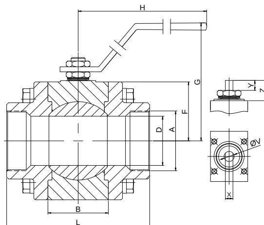
FIG.K 809 SGSGV CL600 2"-2 1/2" BSPP
