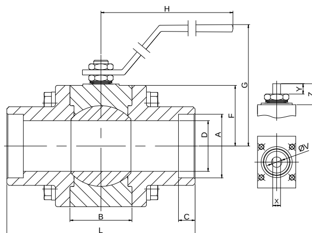
FIG.K 806 SGSGV CL600 2"-2 1/2" SW
