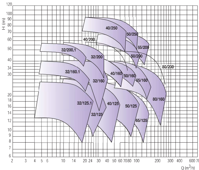
NKP 2 900 tr/min
